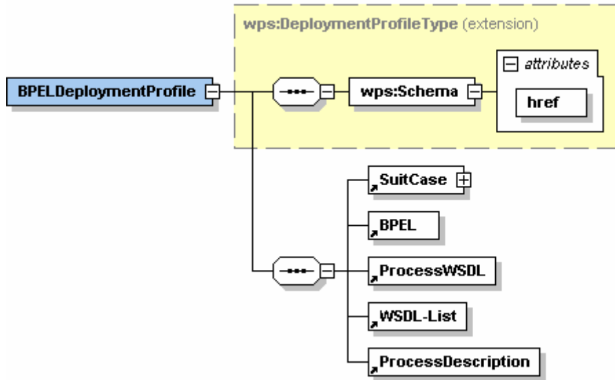
Figure 8: BPELDeploymentProfile Structure.
